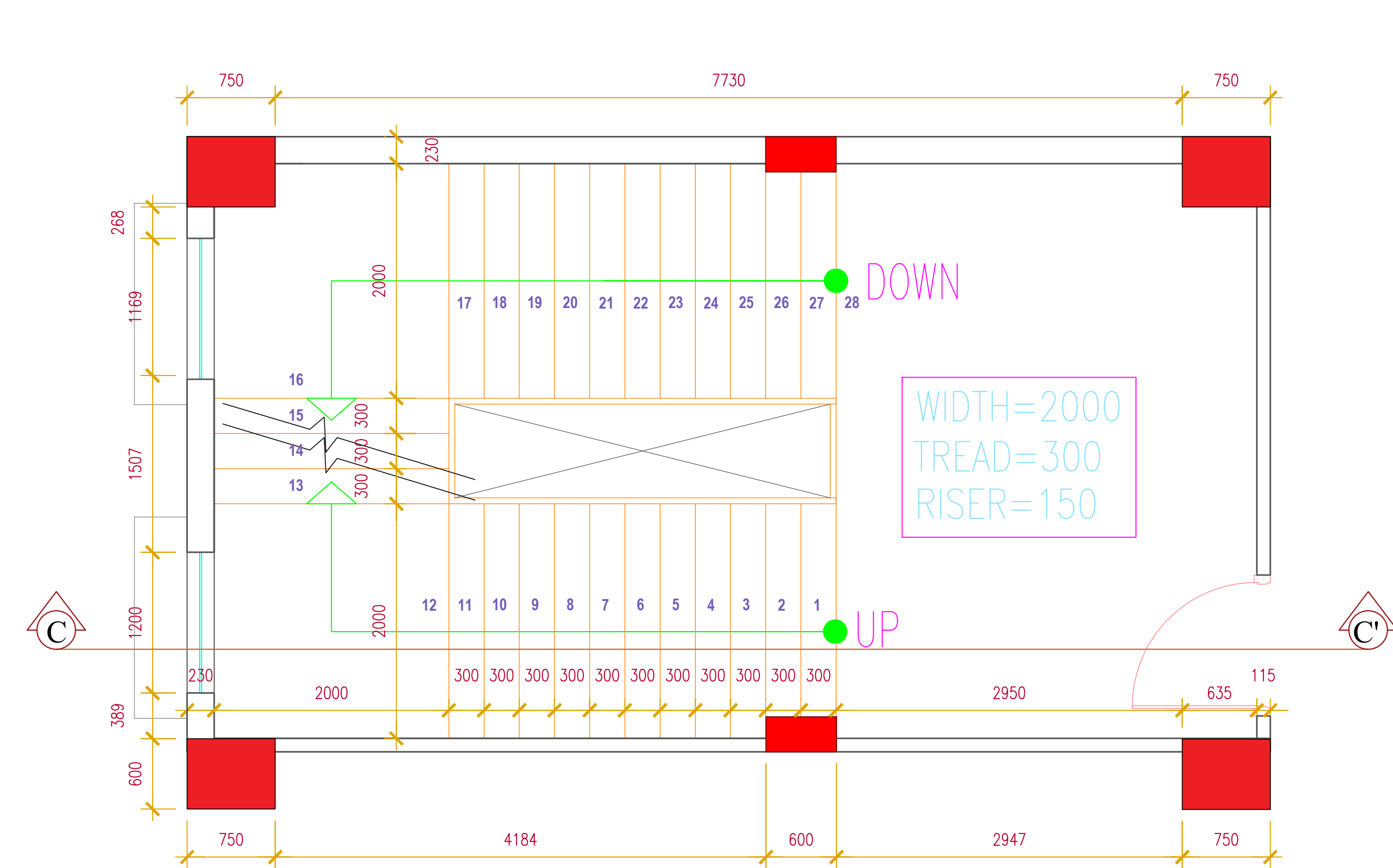
FOURTH FLOOR PLAN (STAIRCASE DETAIL)
