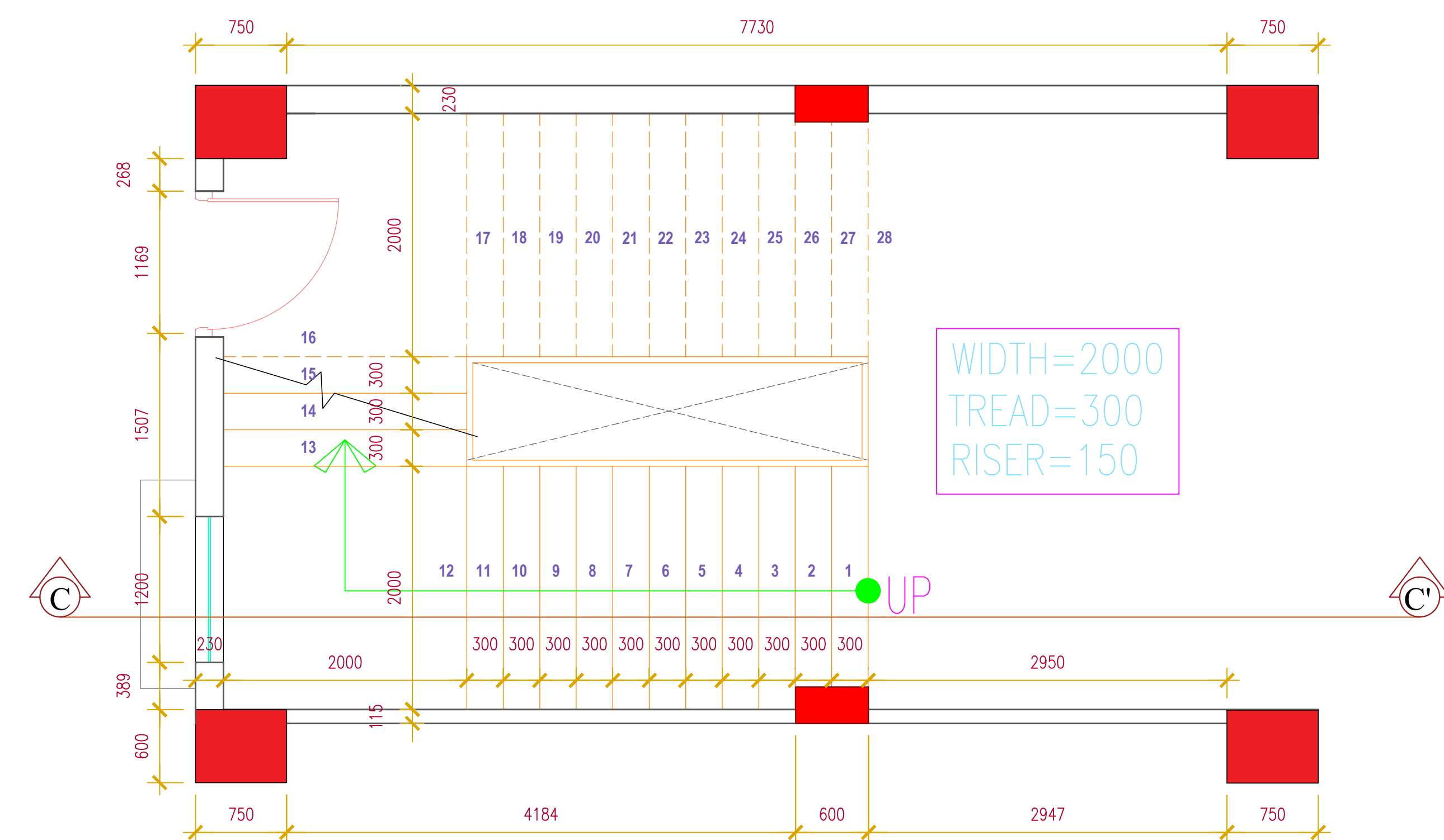
GROUND FLOOR PLAN (STAIRCASE DETAIL)
