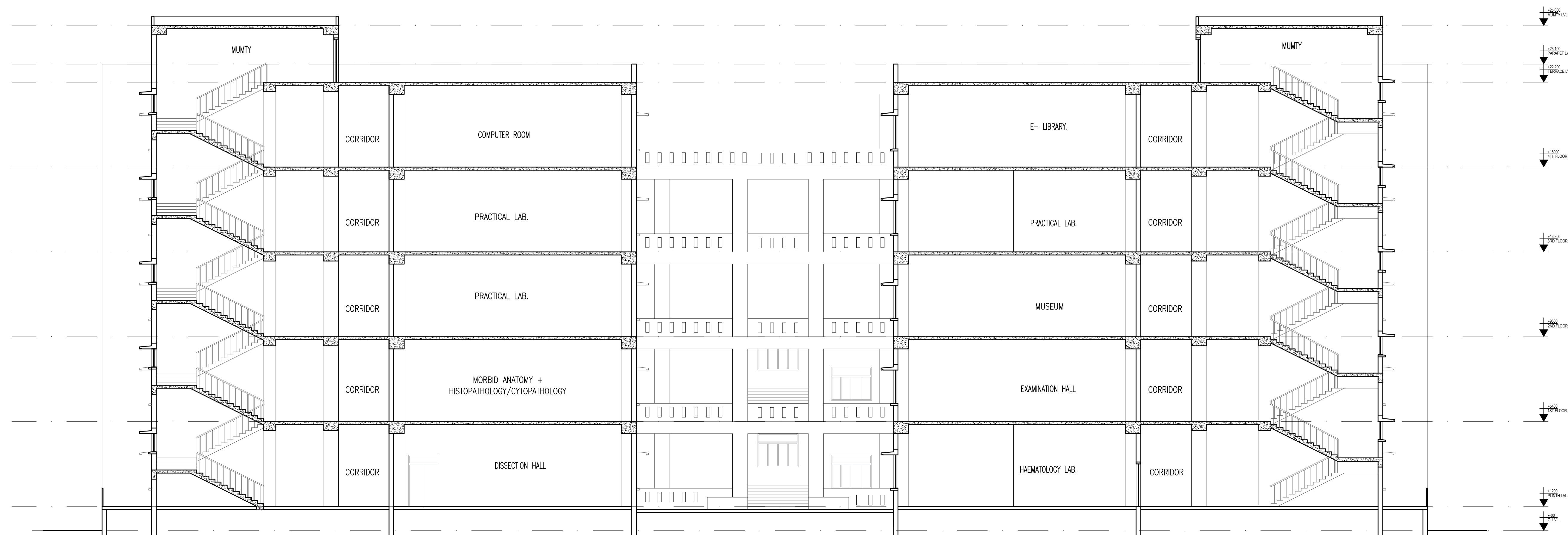
SECTION AT B-B'
