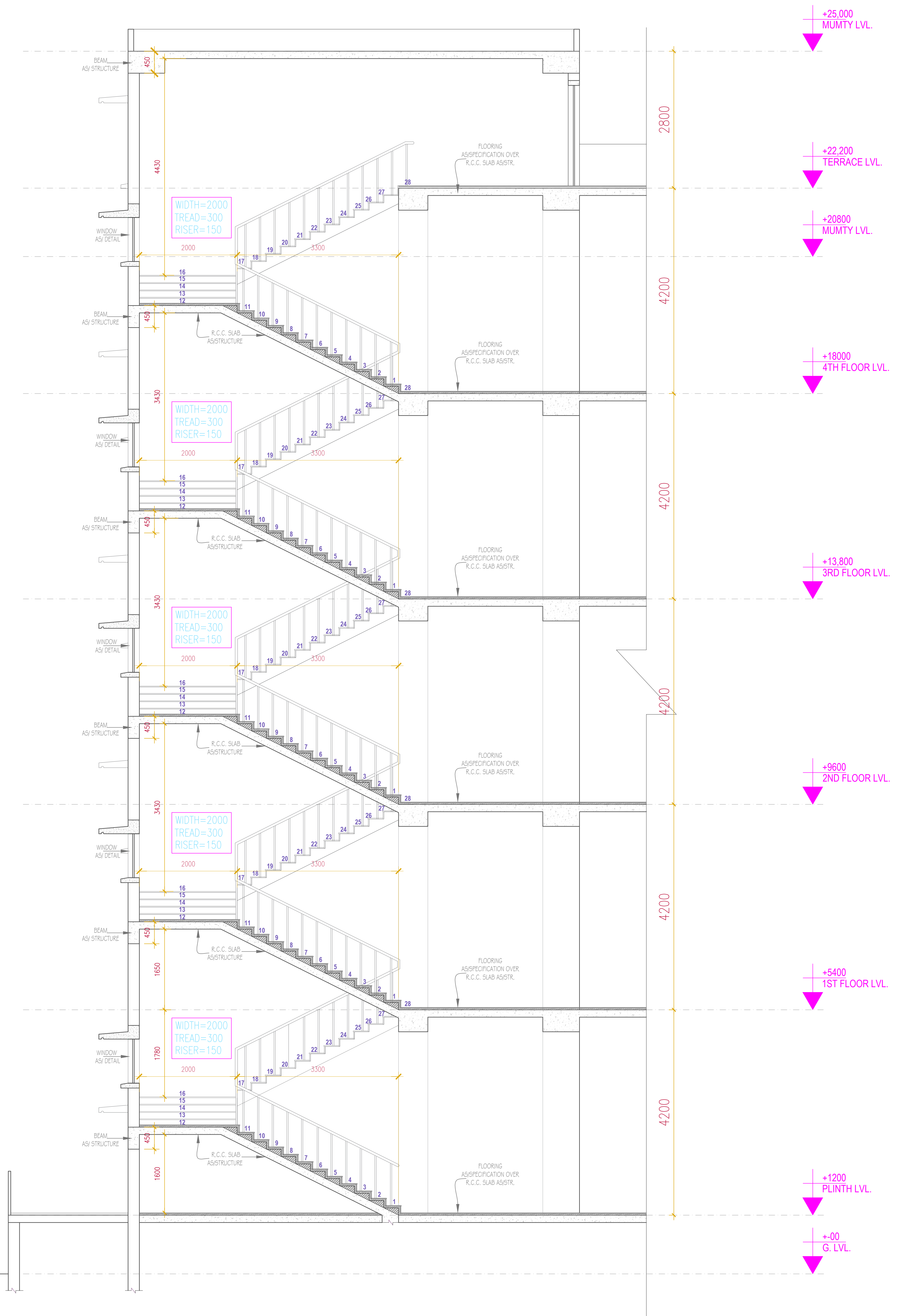
SECTION AT C-C' (STAIRCASE DETAIL)
