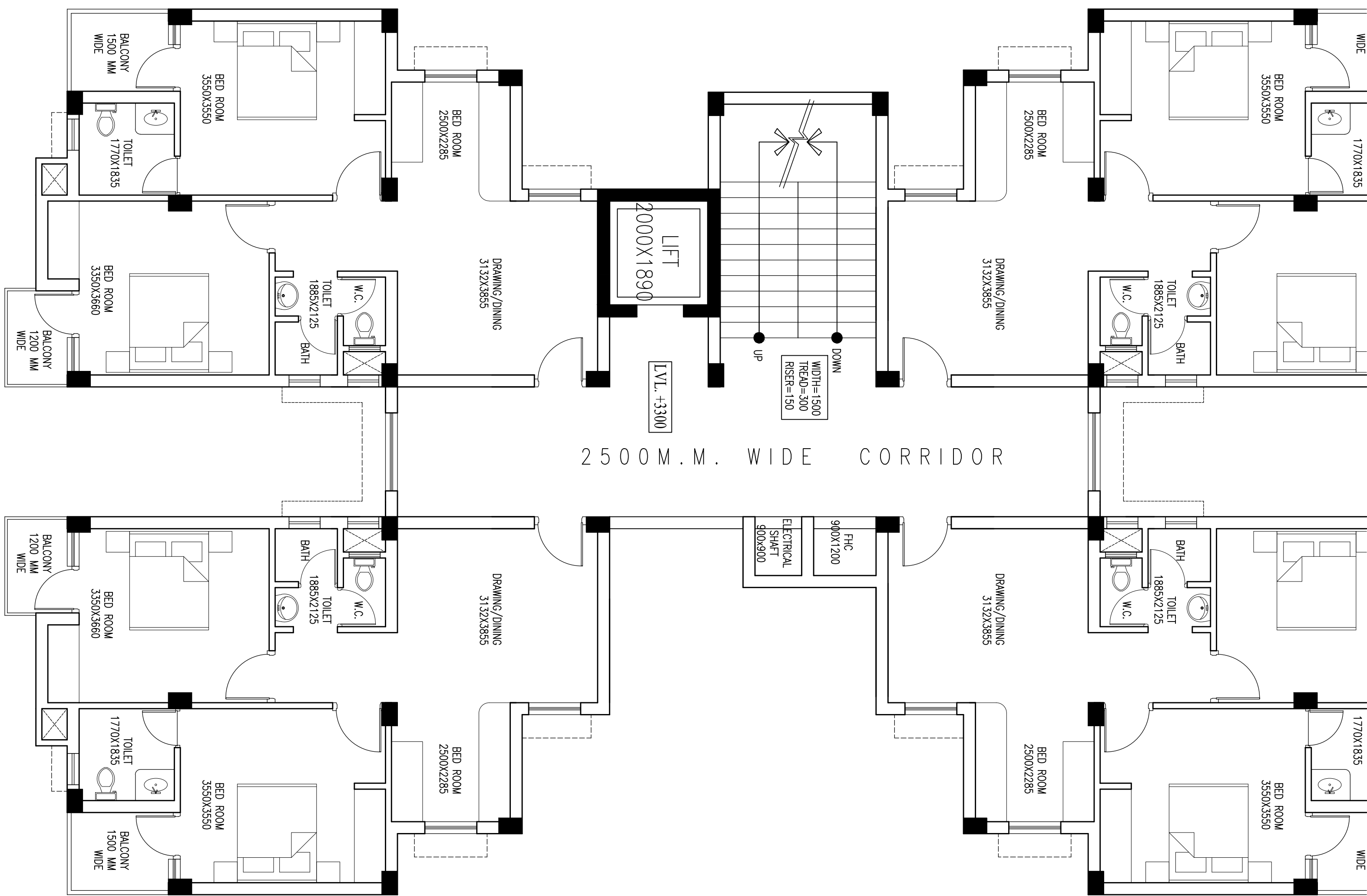
FIRST- FIFTH FLOOR PLAN
