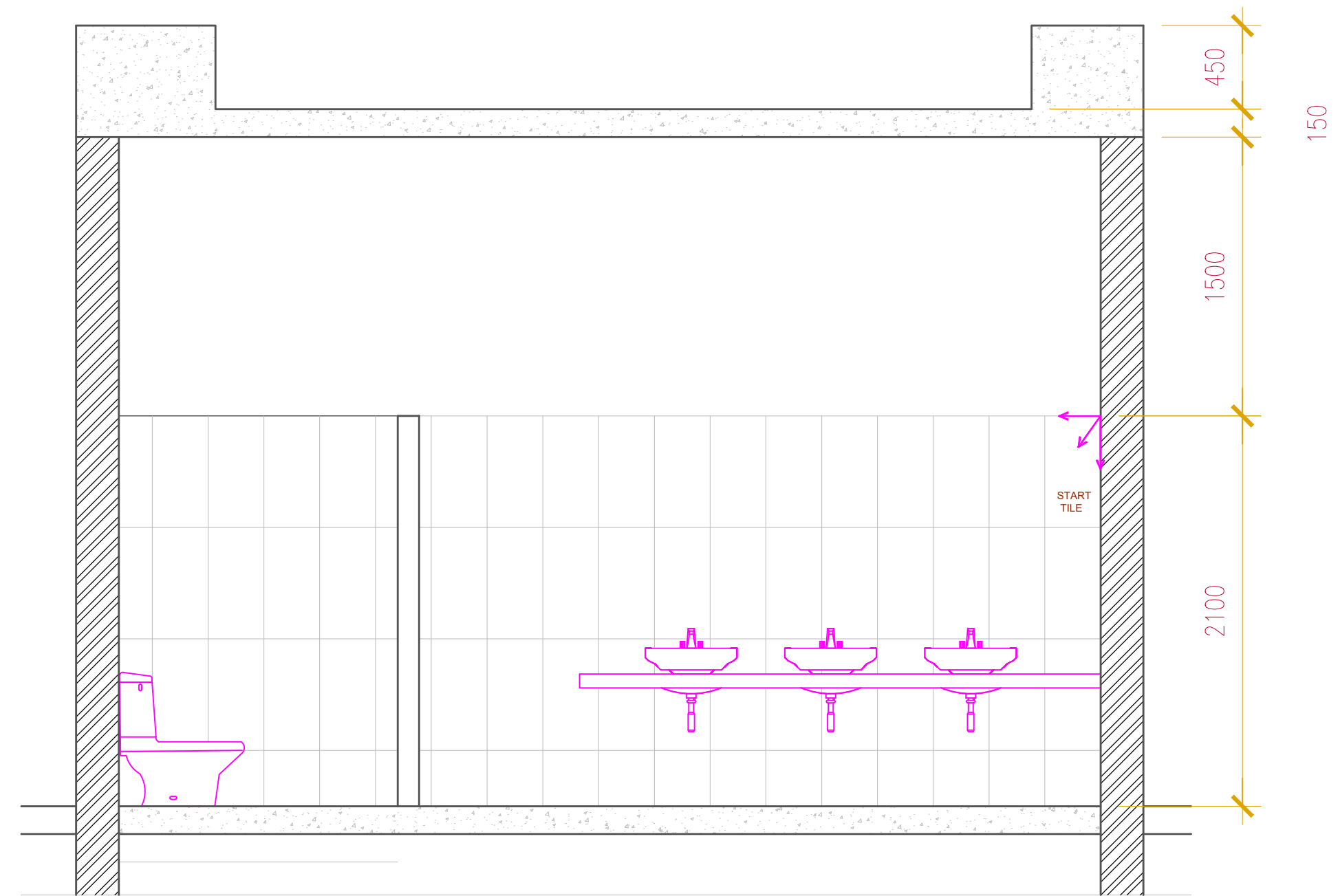
ELEVATION 2 FOR T1
