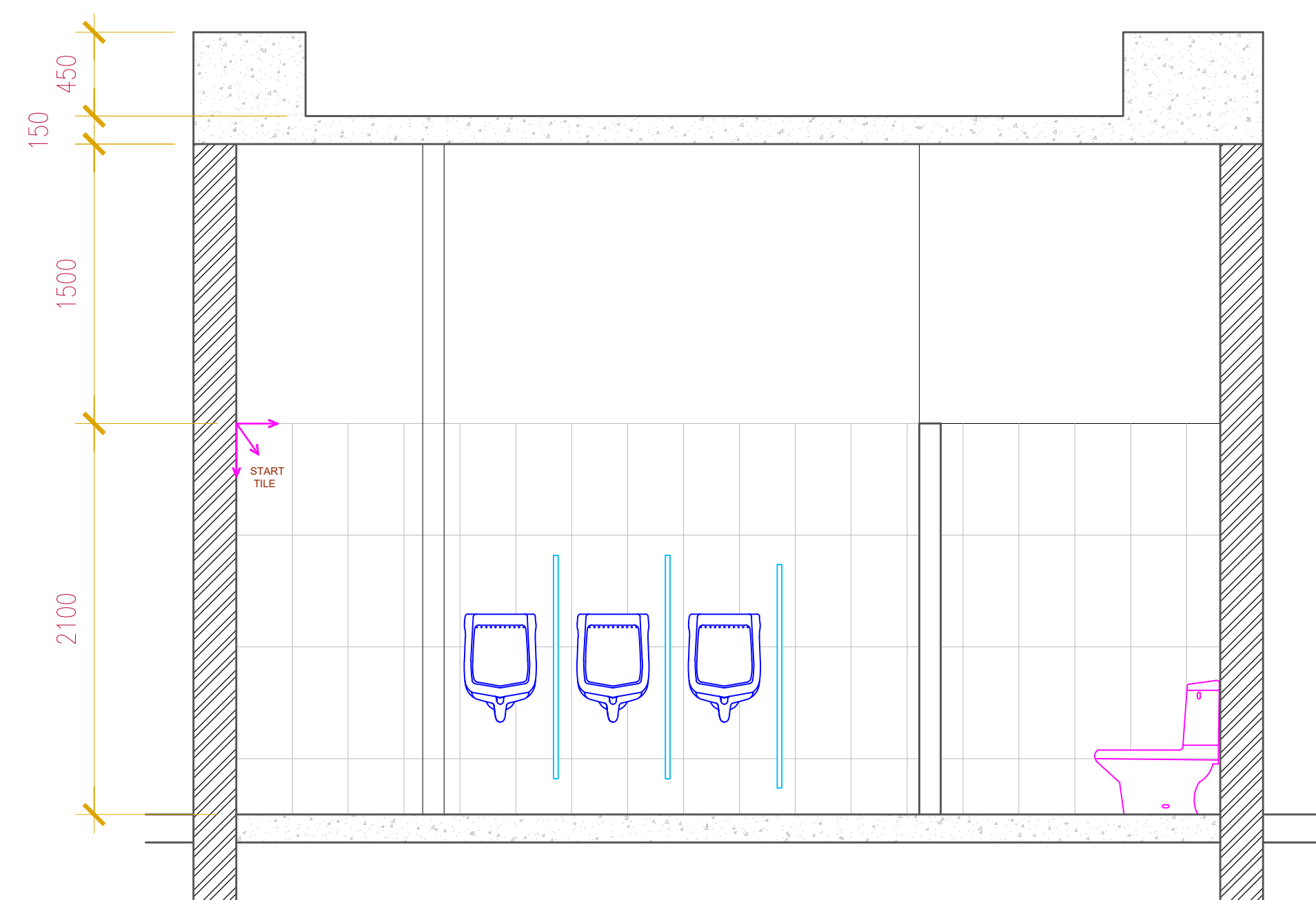
ELEVATION 4 FOR T1
