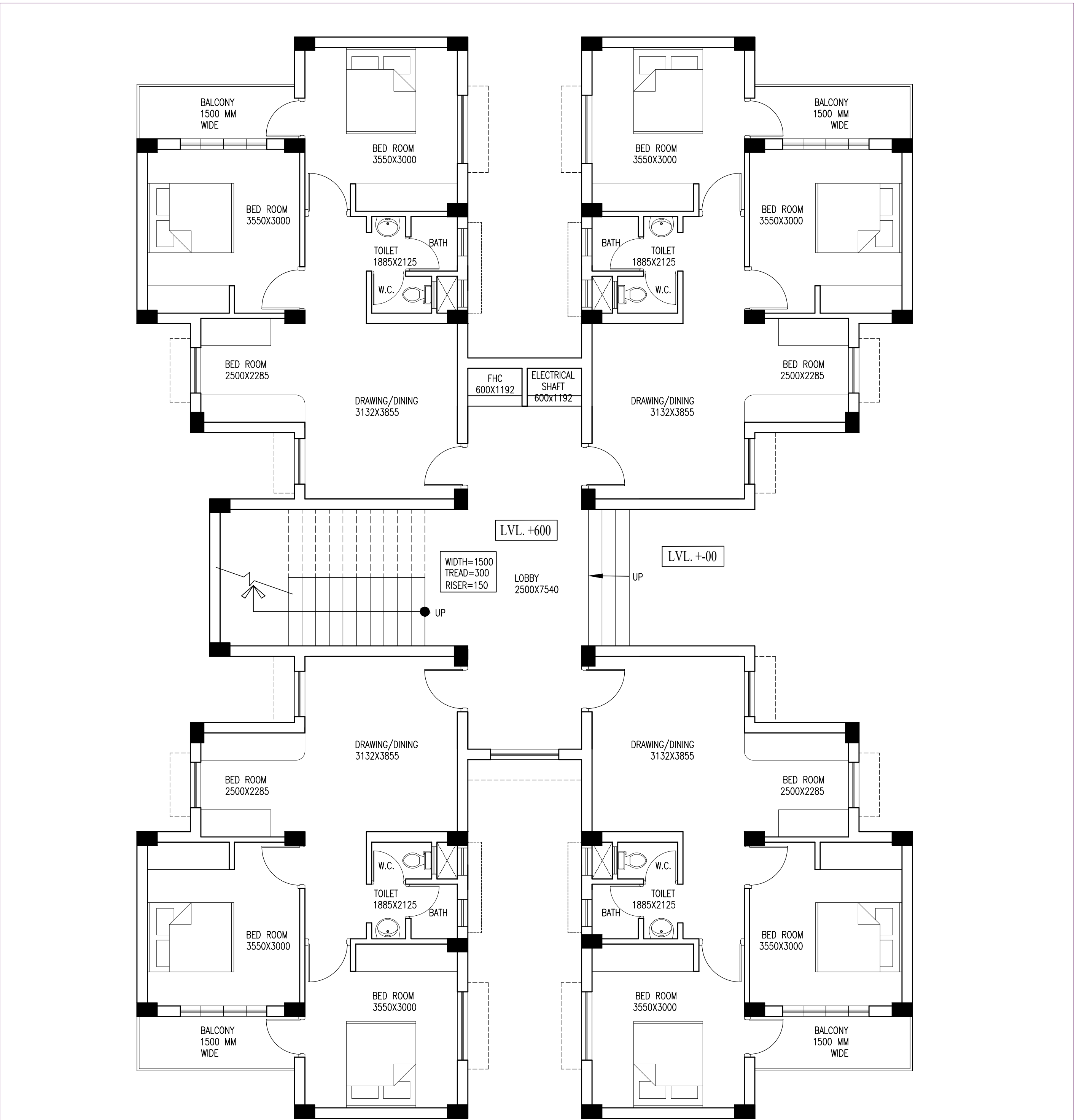
TYPE- 2 HOUSING
