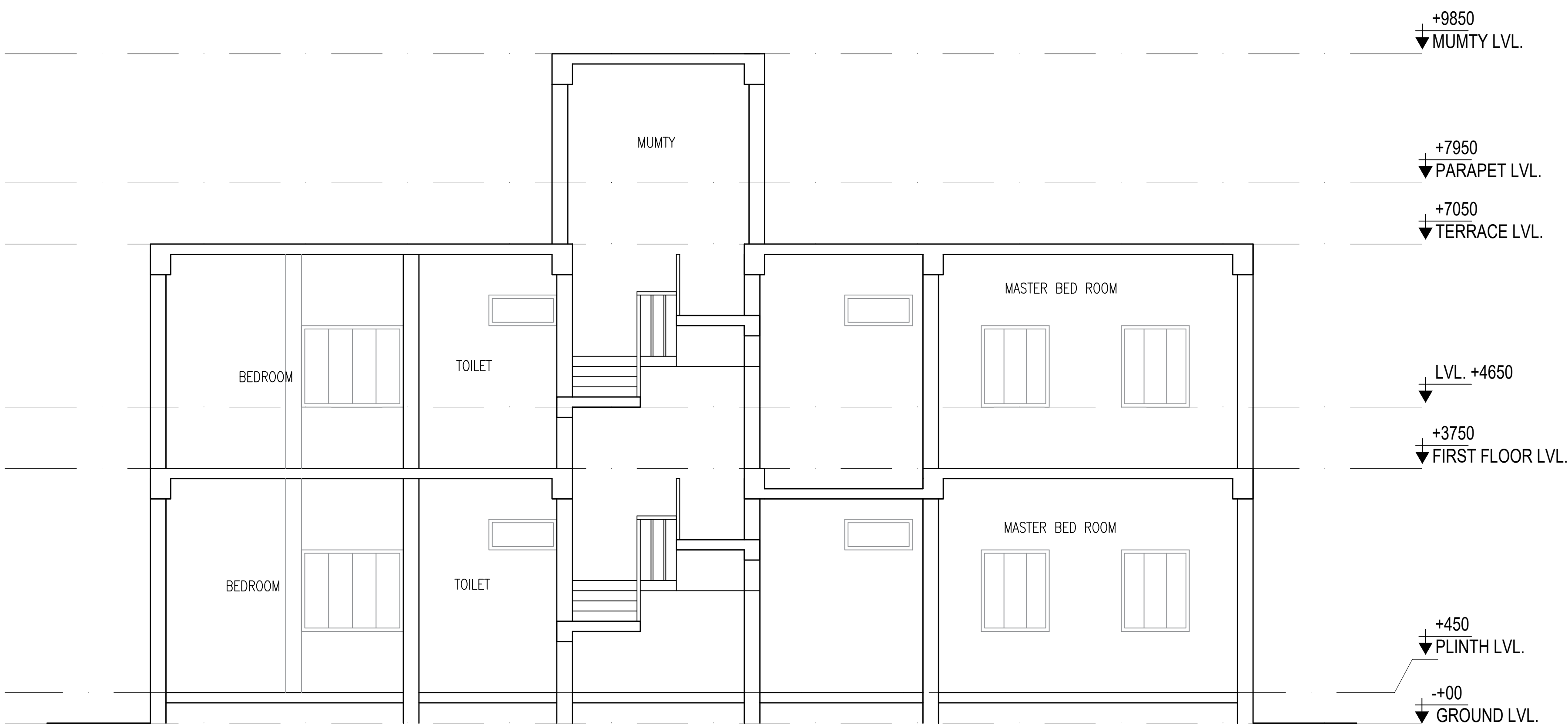
SECTION AT F-F'
