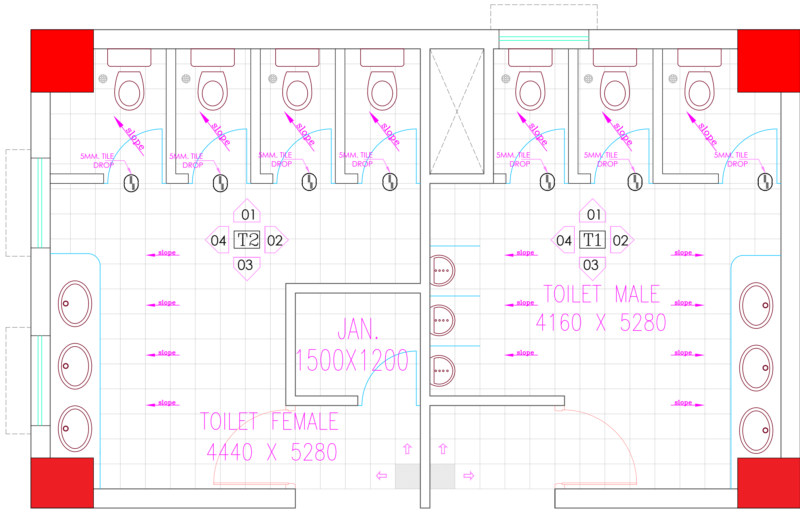
GROUND FLOOR (TOILET DETAIL) FLOORING
