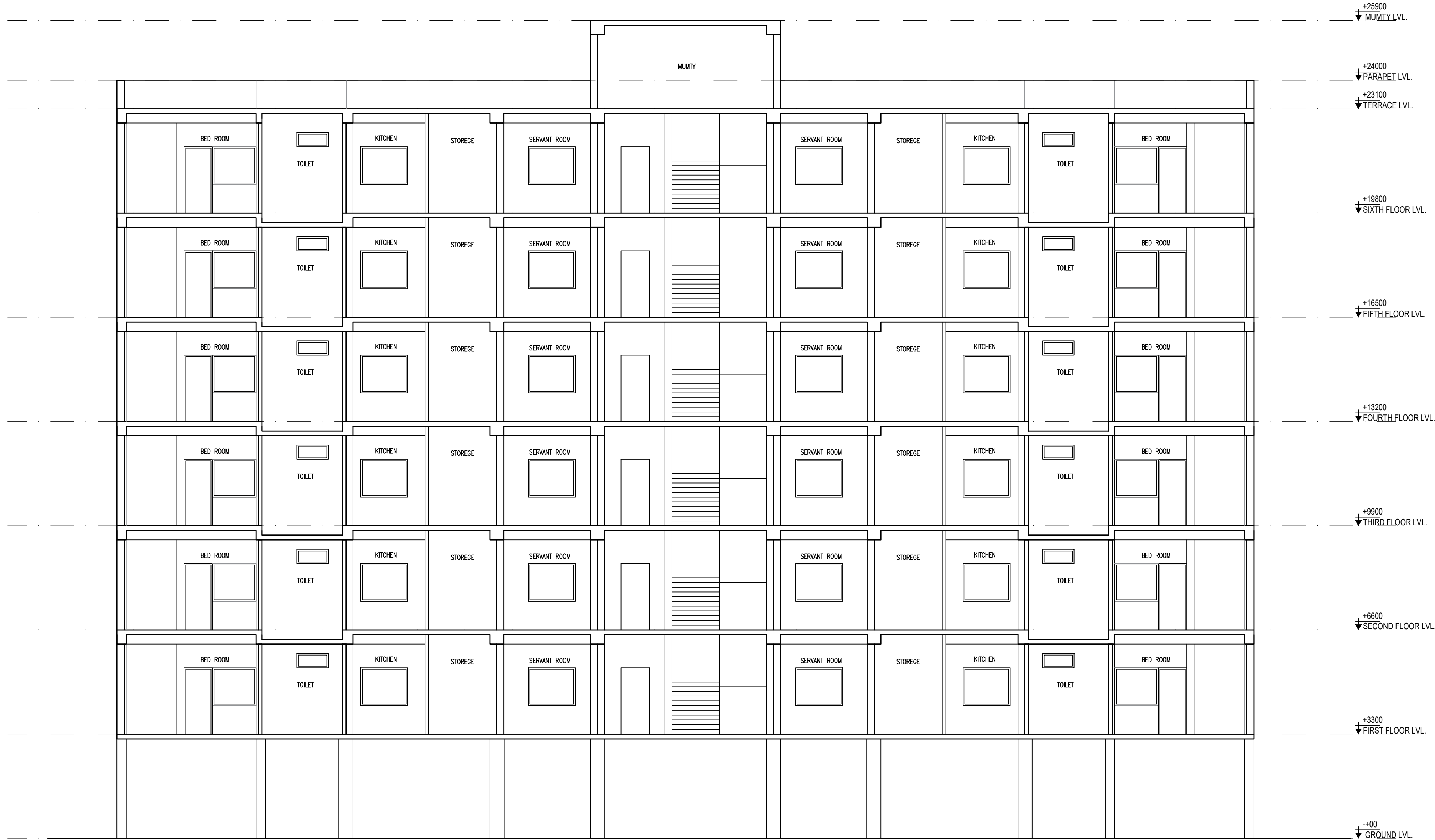
SECTION AT G-G'
