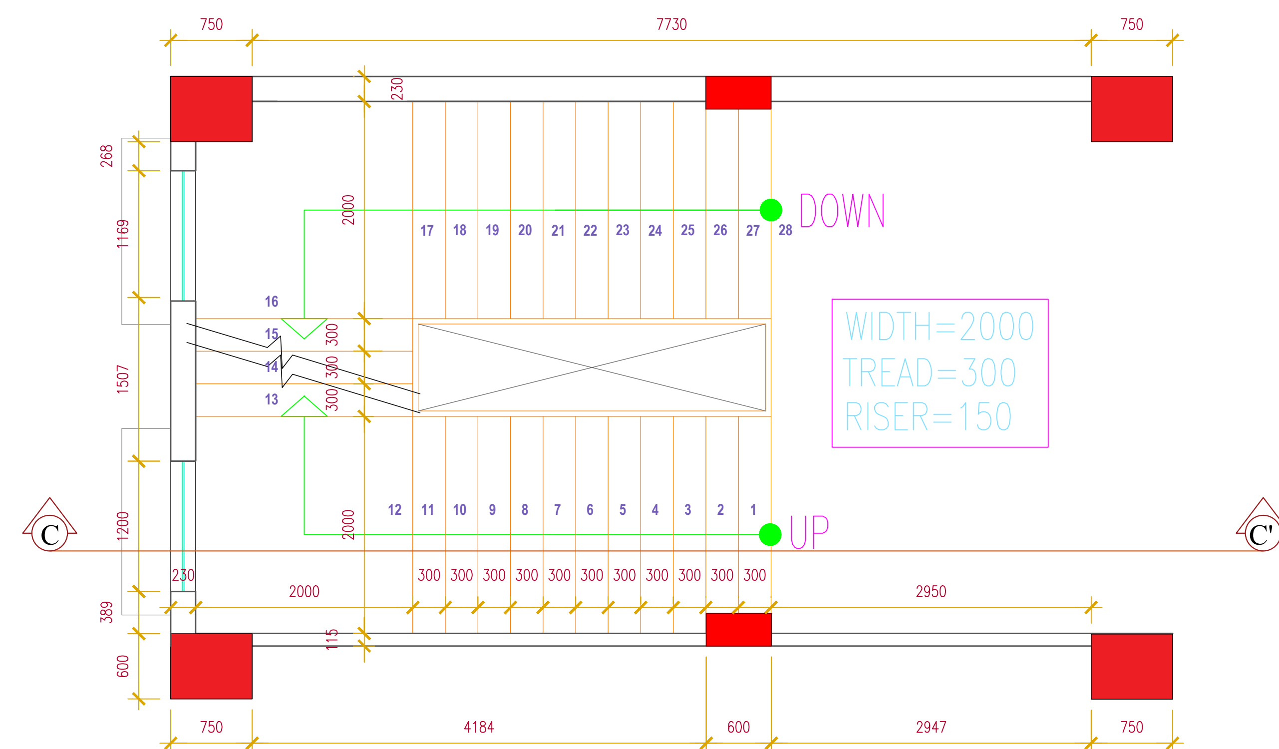
FIRST-THIRD FLOOR PLAN (STAIRCASE DETAIL)
